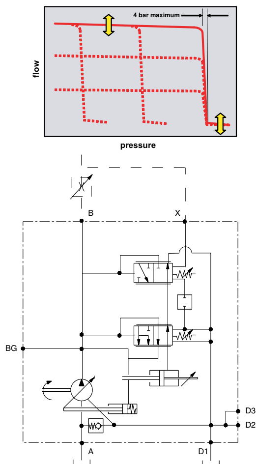
Load Sensing and Pressure Limiter Control with Optional Minimum & Maximum Displacement Adjustments and Case-to-Inlet Check Valve (A minimum displacement stop requires the use of a system relief valve.)
