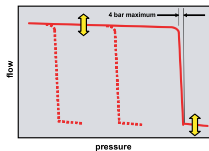
pilot-operated pressure limiter control with minimum displacement stop
